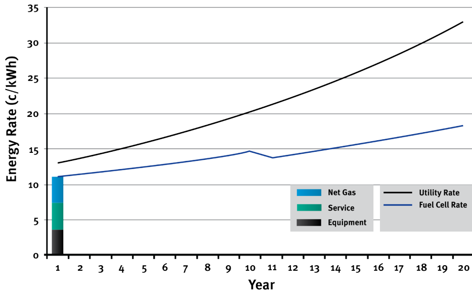
PureCell System Cost of Energy vs. Utility
